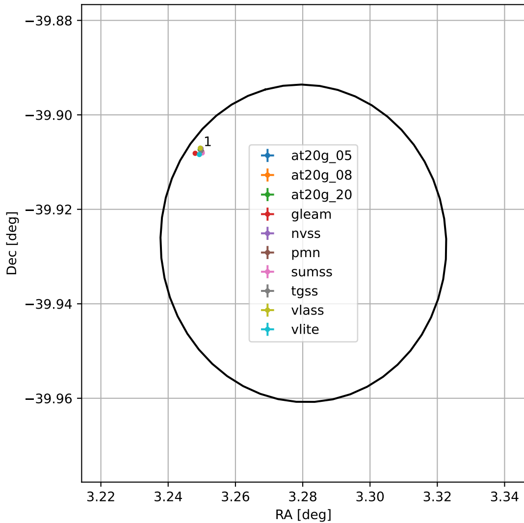
4FGL J0013.1-3955
