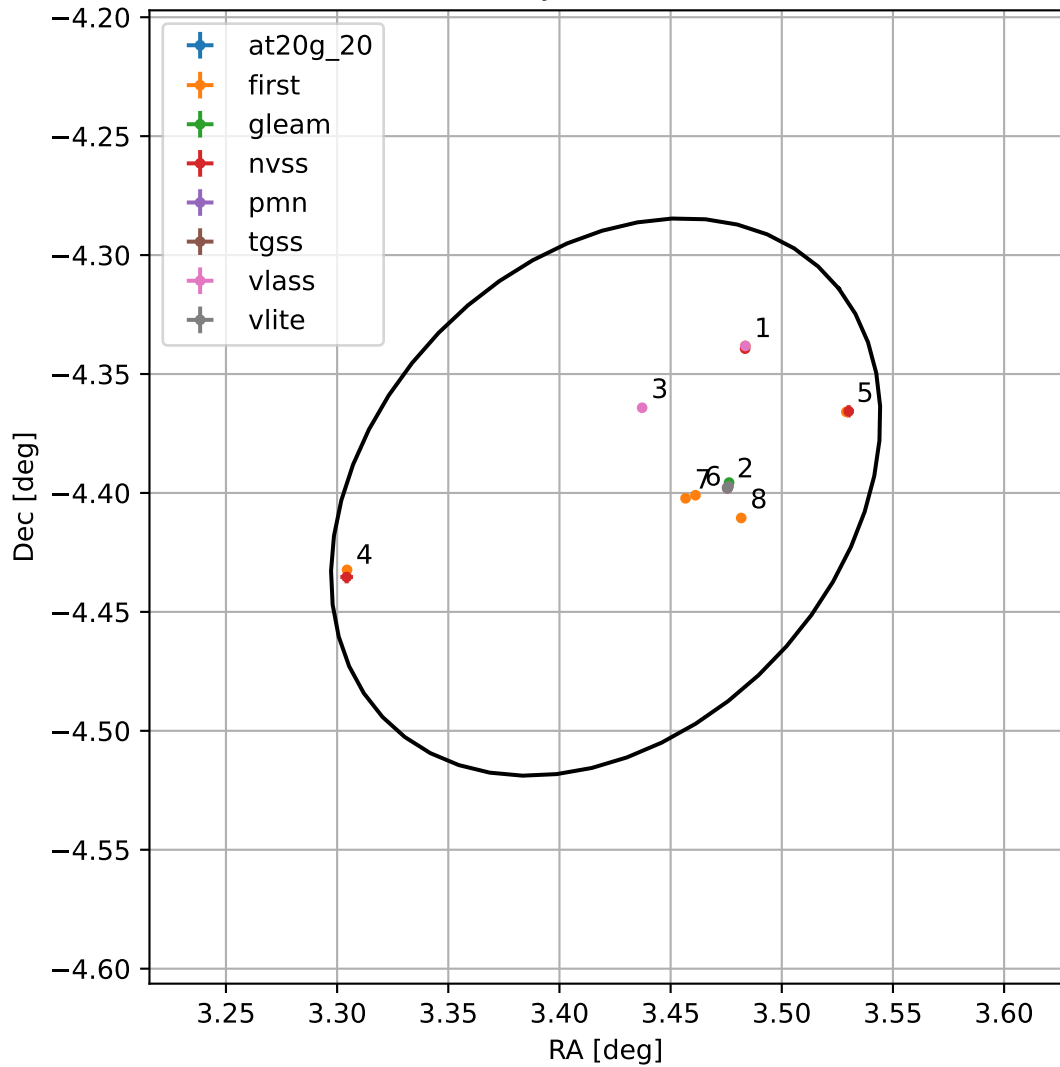
4FGL J0013.6-0424
