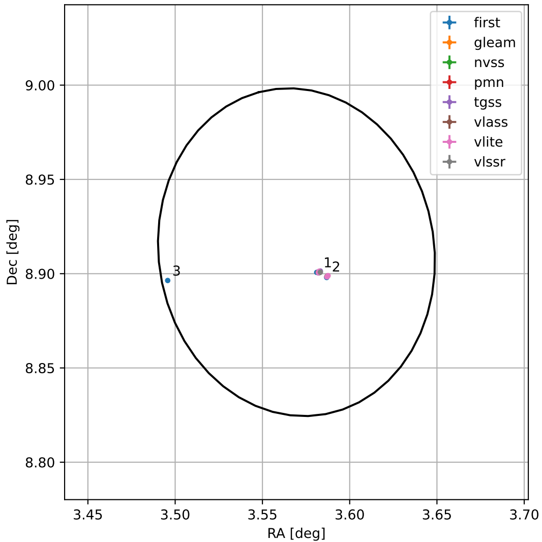
4FGL J0014.2+0854
