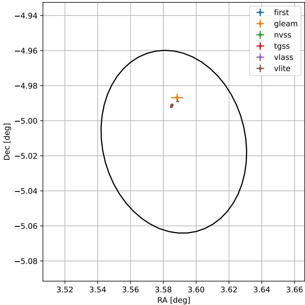
4FGL J0014.3-0500
