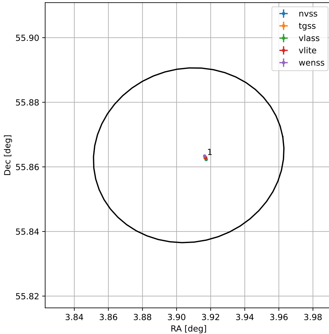
4FGL J0015.6+5551
