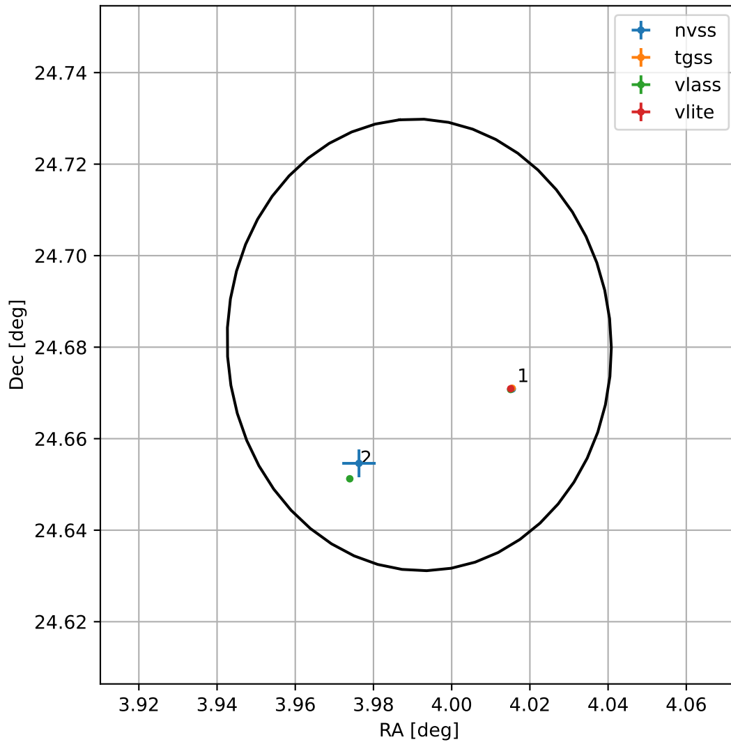
4FGL J0015.9+2440
