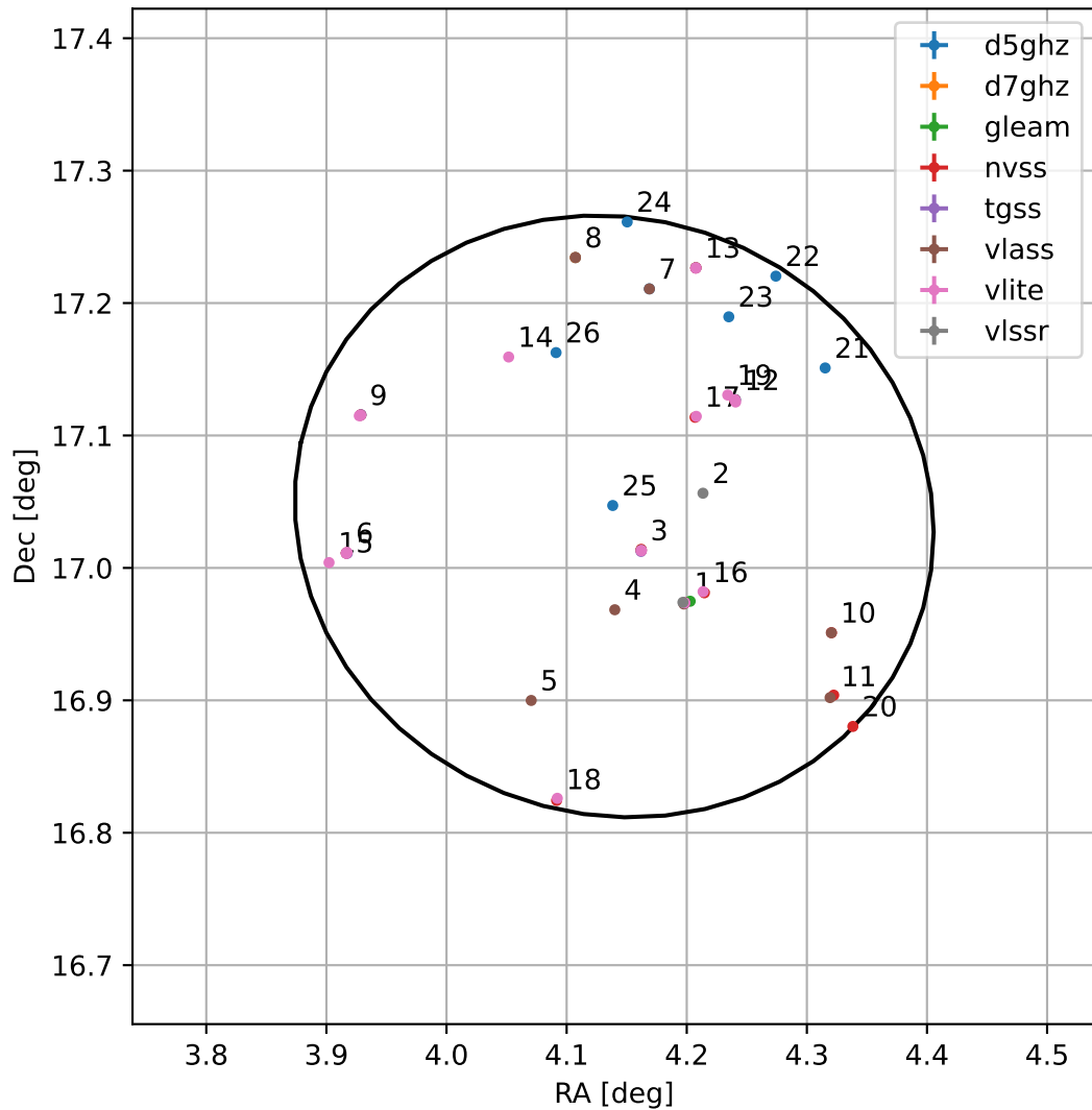
4FGL J0016.5+1702
