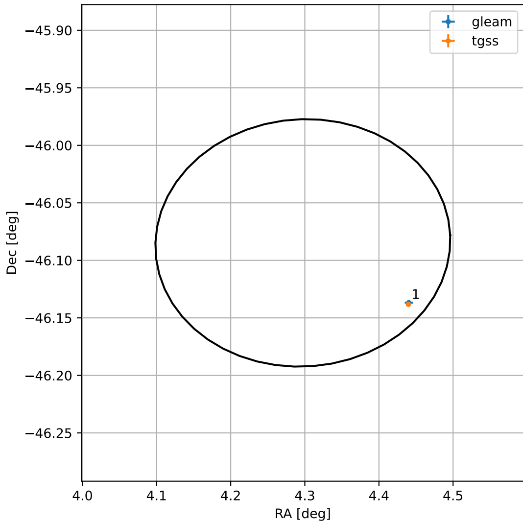
4FGL J0017.1-4605
