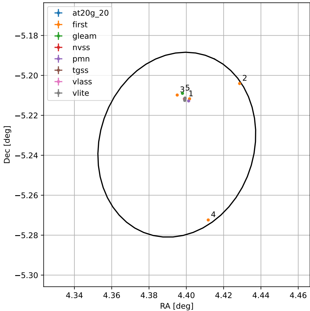
4FGL J0017.5-0514
