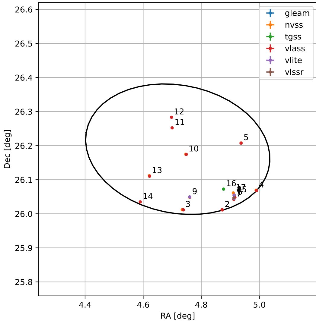
4FGL J0018.8+2611
