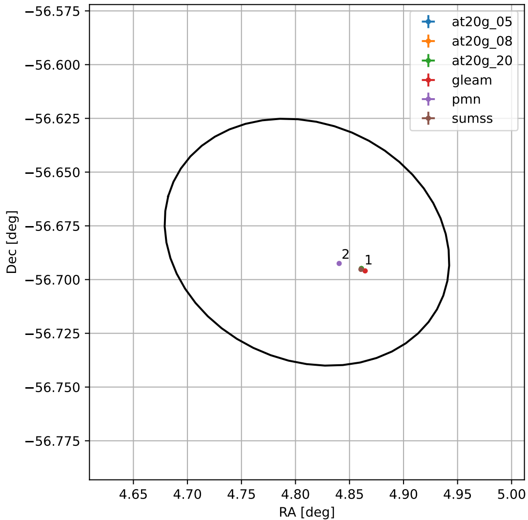
4FGL J0019.2-5640
