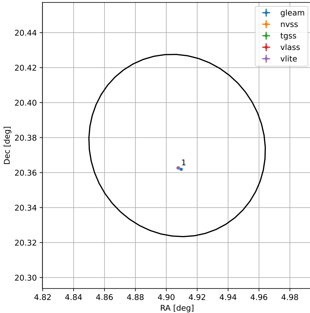
4FGL J0019.6+2022
