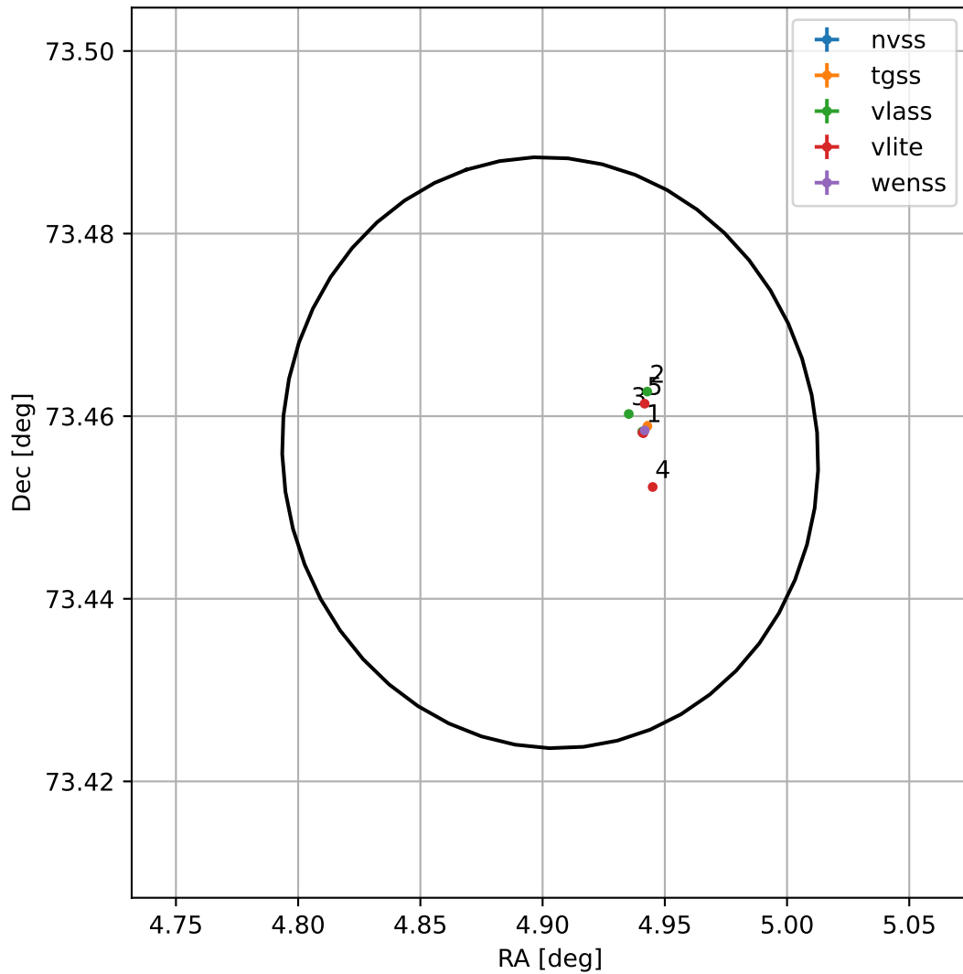
4FGL J0019.6+7327
