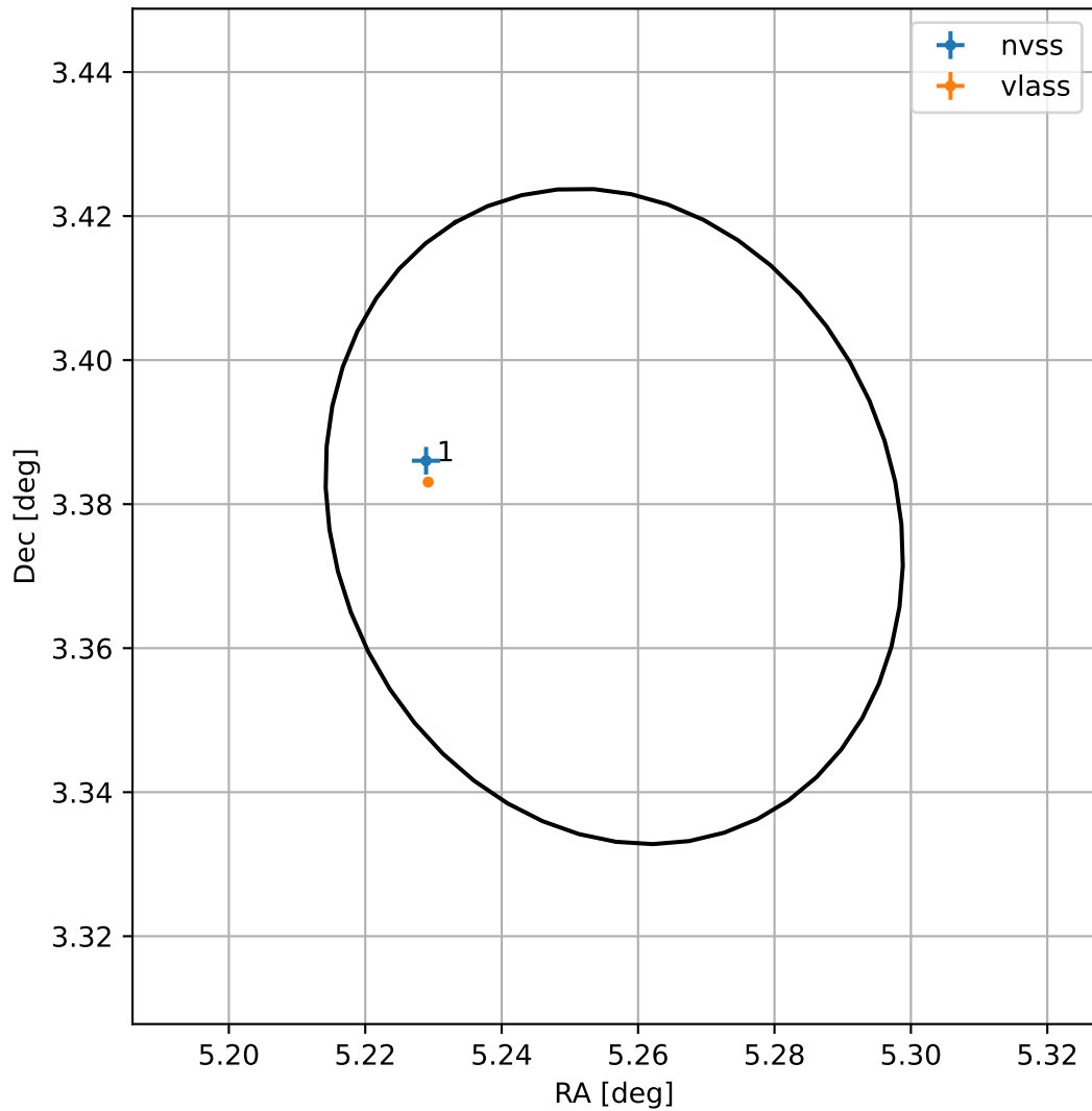
4FGL J0021.0+0322
