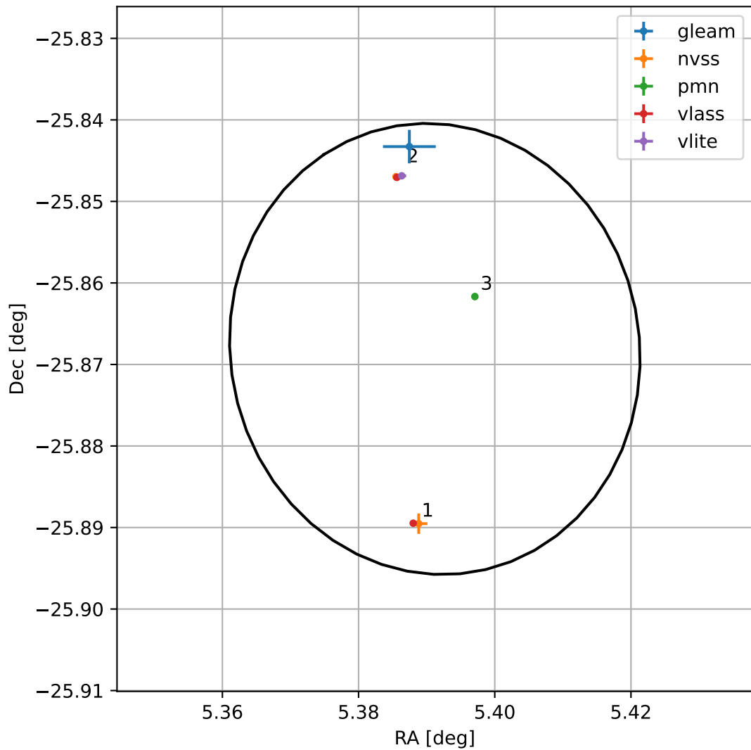
4FGL J0021.5-2552
