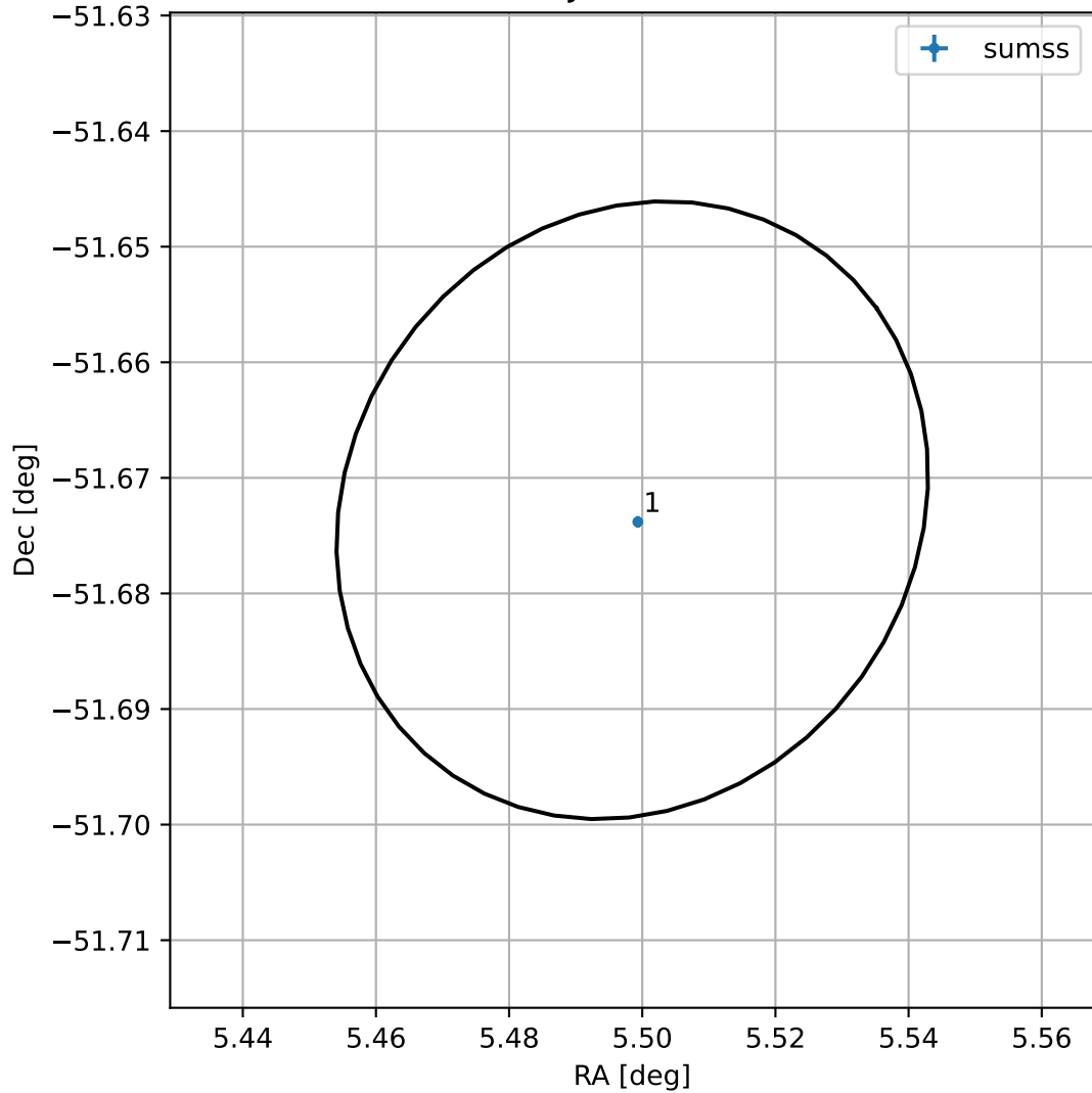
4FGL J0021.9-5140
