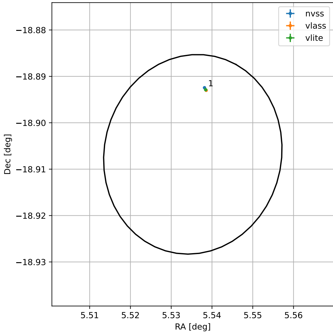
4FGL J0022.1-1854
