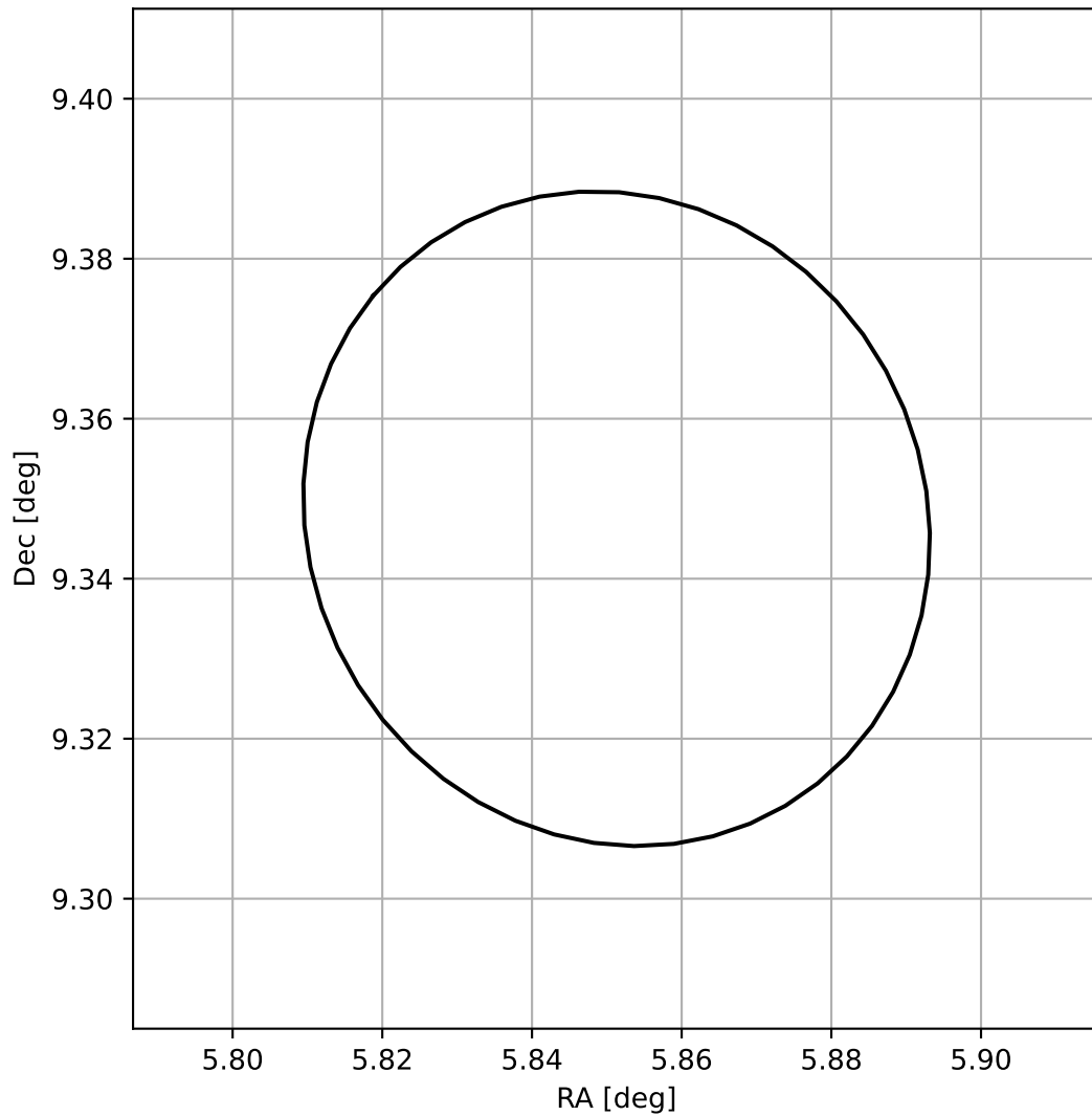
4FGL J0023.4+0920
