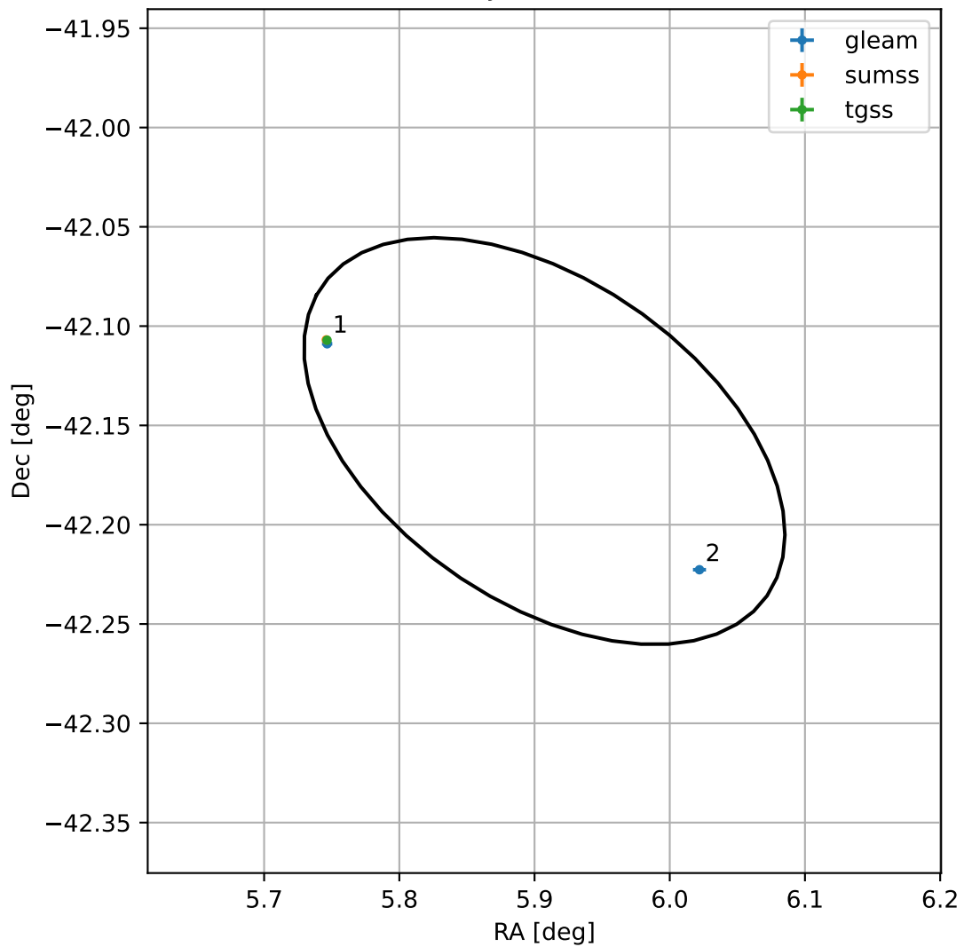
4FGL J0023.6-4209
