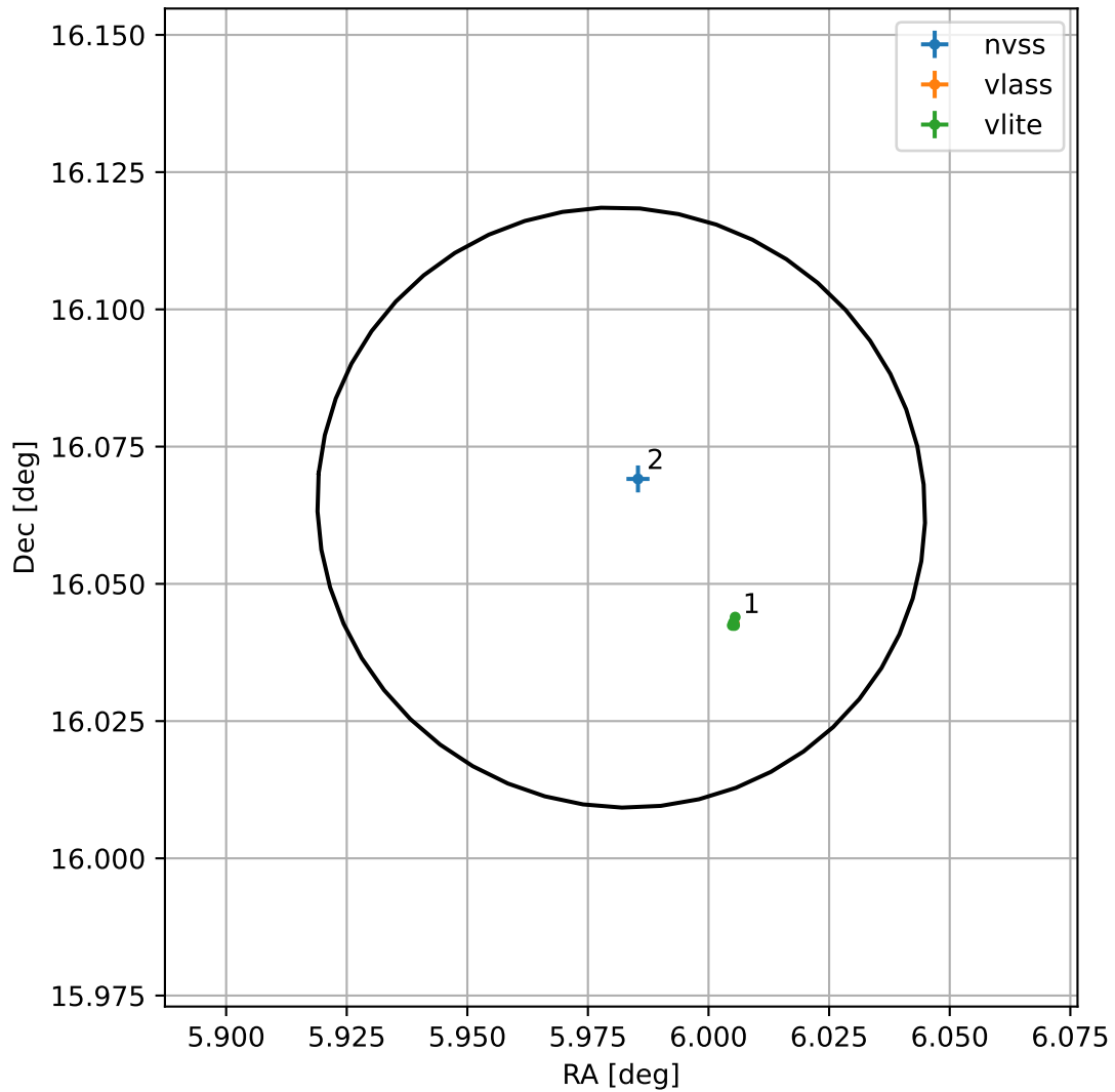
4FGL J0023.9+1603
