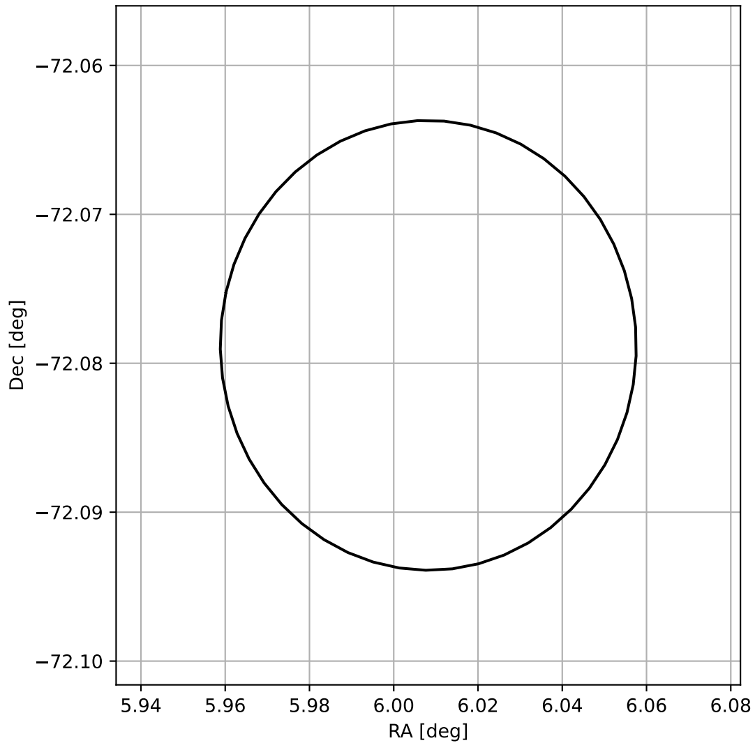
4FGL J0024.0-7204
