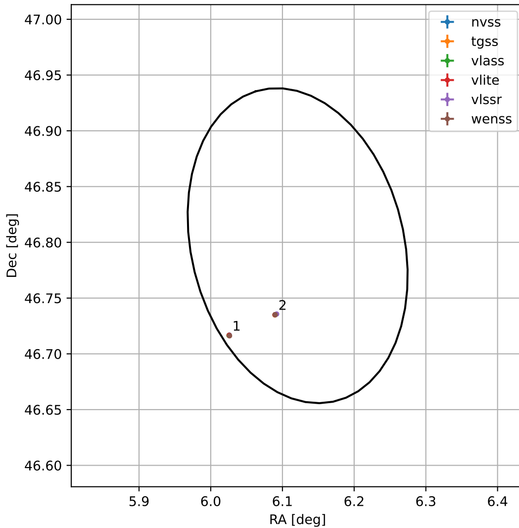
4FGL J0024.4+4647
