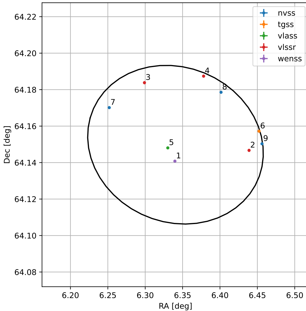
4FGL J0025.3+6408
