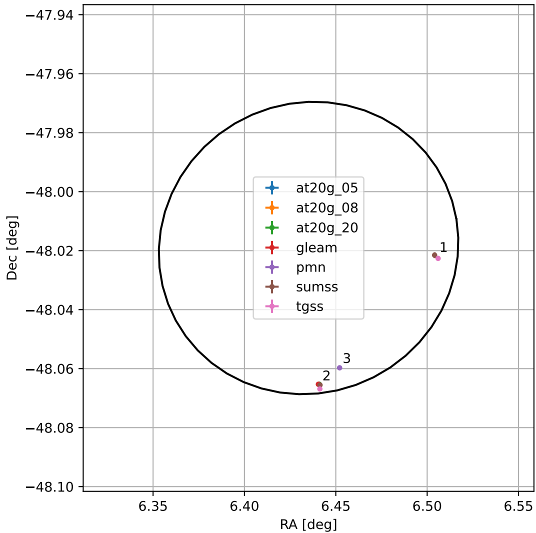
4FGL J0025.7-4801
