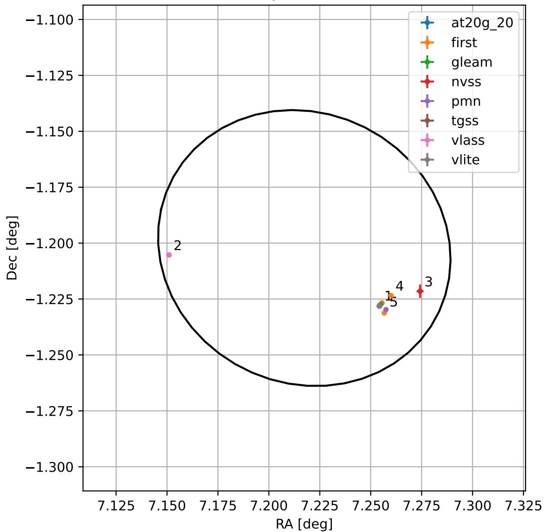
4FGL J0028.8-0112
