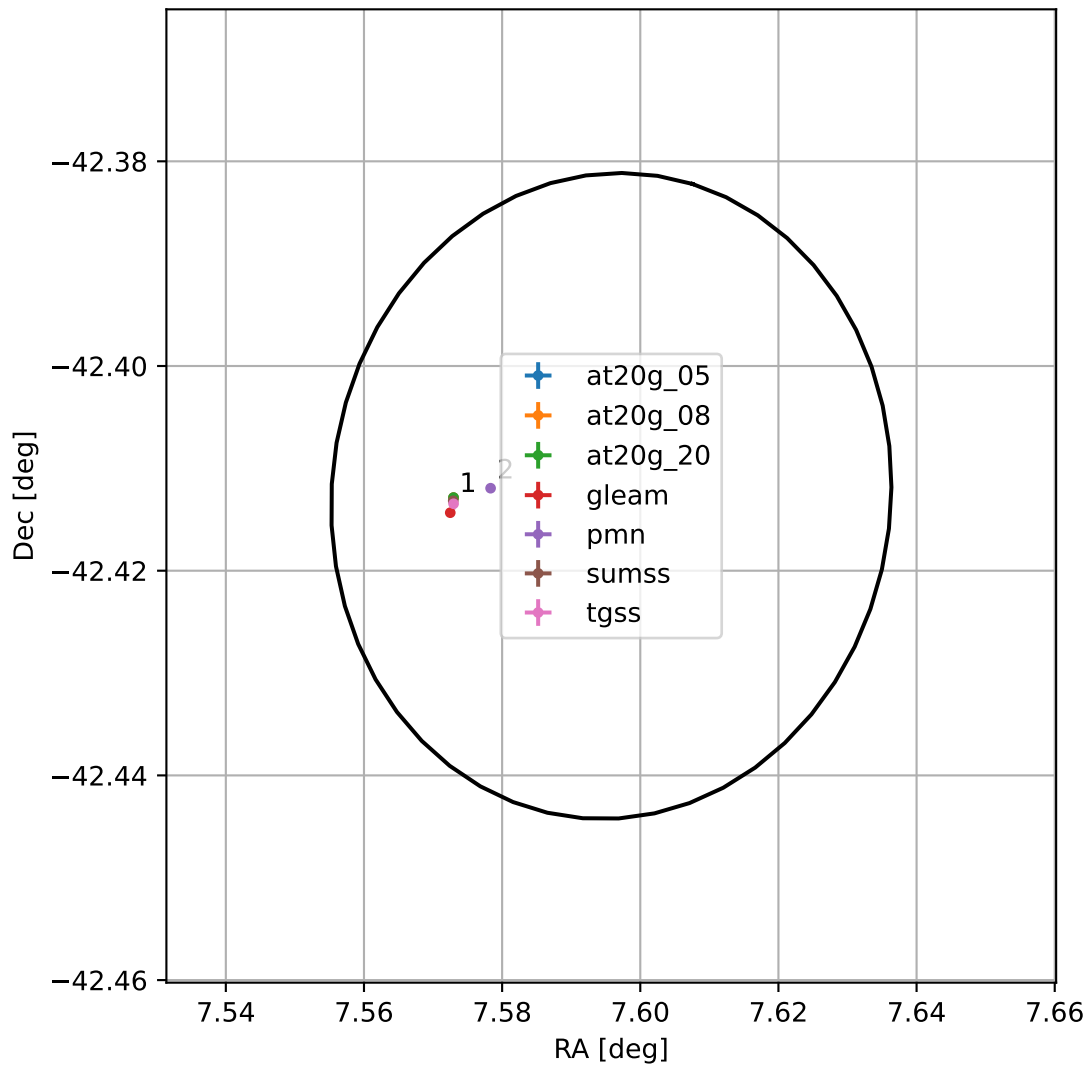
4FGL J0030.3-4224
