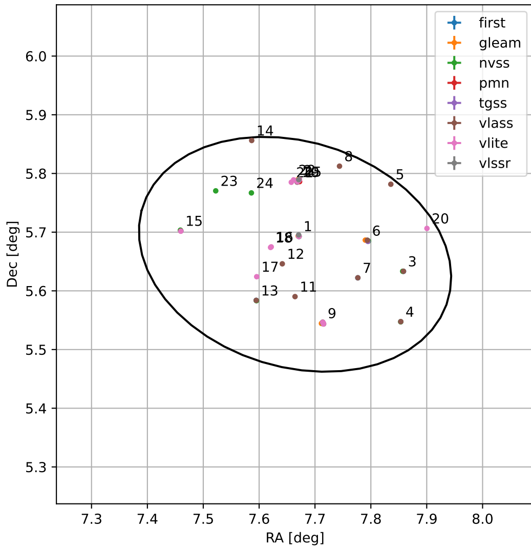
4FGL J0030.6+0539
