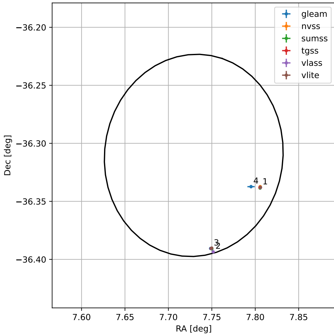
4FGL J0030.9-3618
