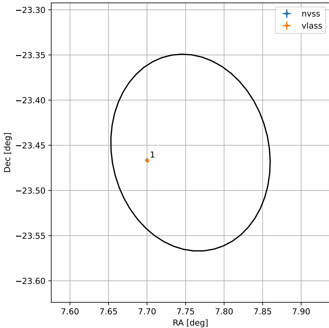
4FGL J0031.0-2327
