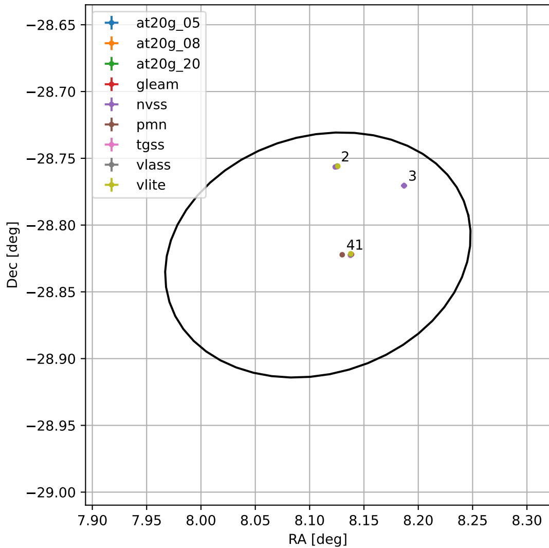
4FGL J0032.4-2849
