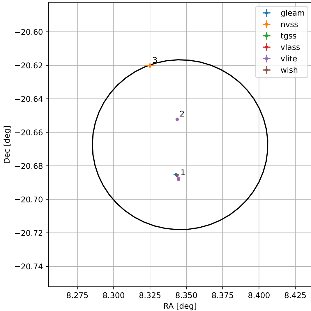
4FGL J0033.3-2040
