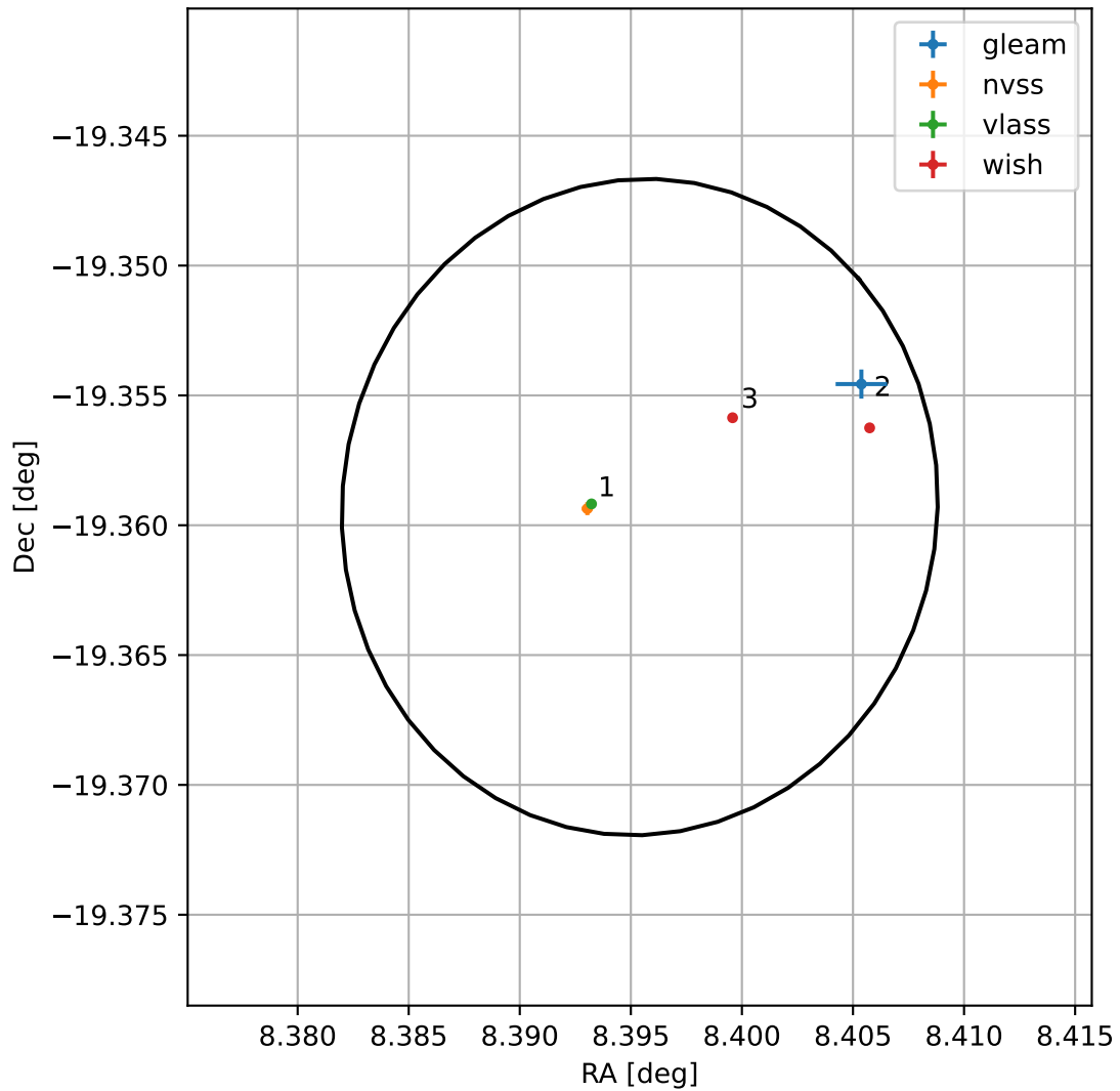
4FGL J0033.5-1921
