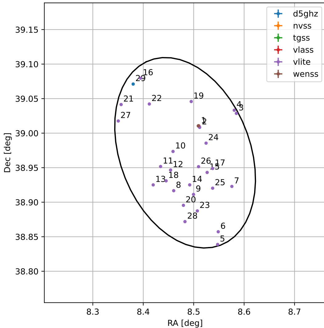
4FGL J0033.9+3858
