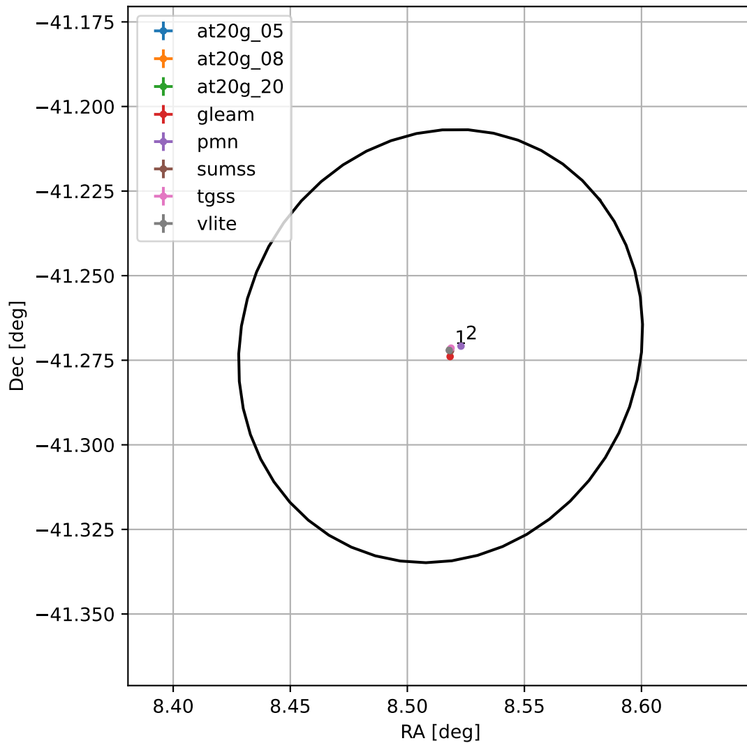
4FGL J0034.0-4116
