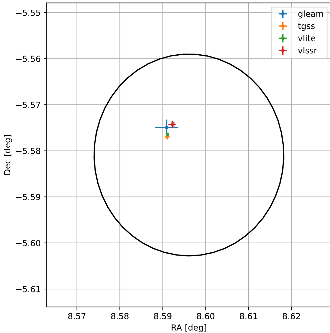
4FGL J0034.3-0534
