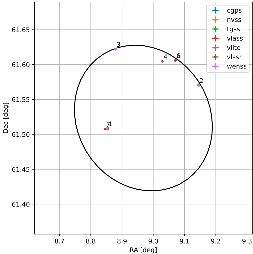
4FGL J0035.8+6131
