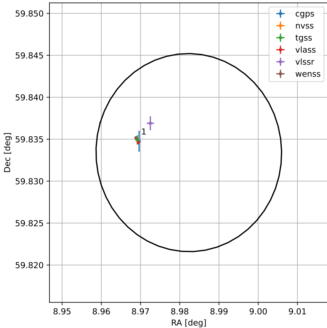
4FGL J0035.9+5950
