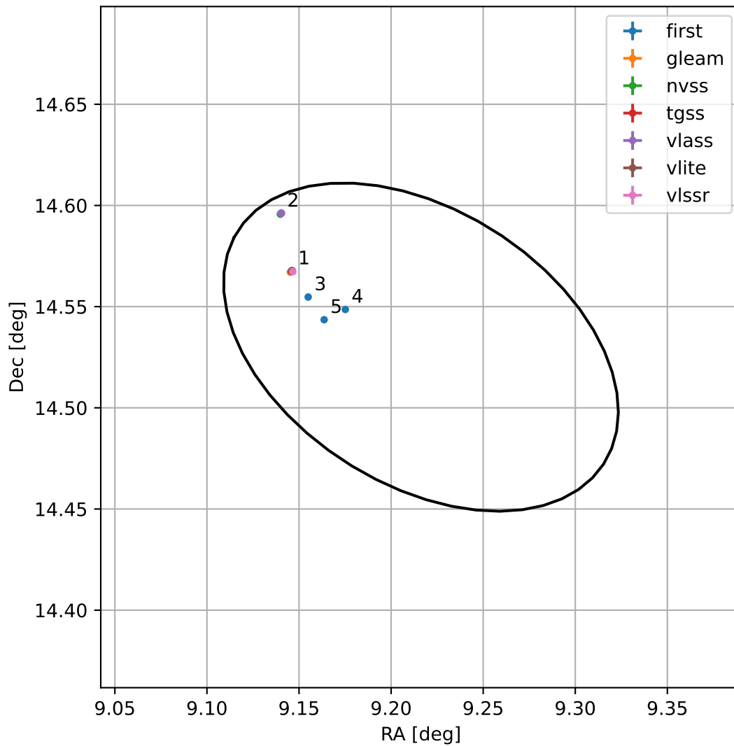
4FGL J0036.8+1431
