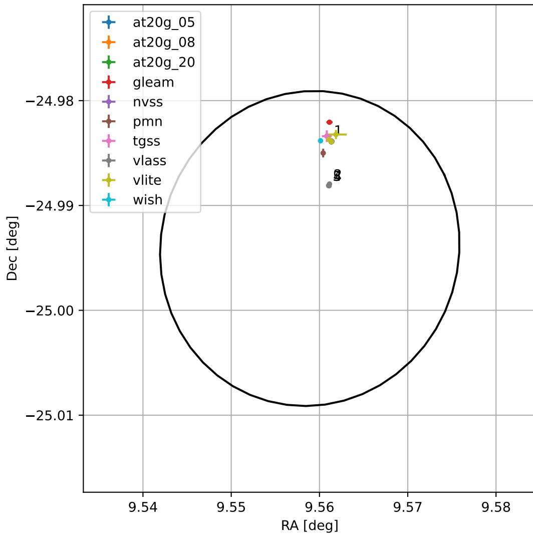
4FGL J0038.2-2459
