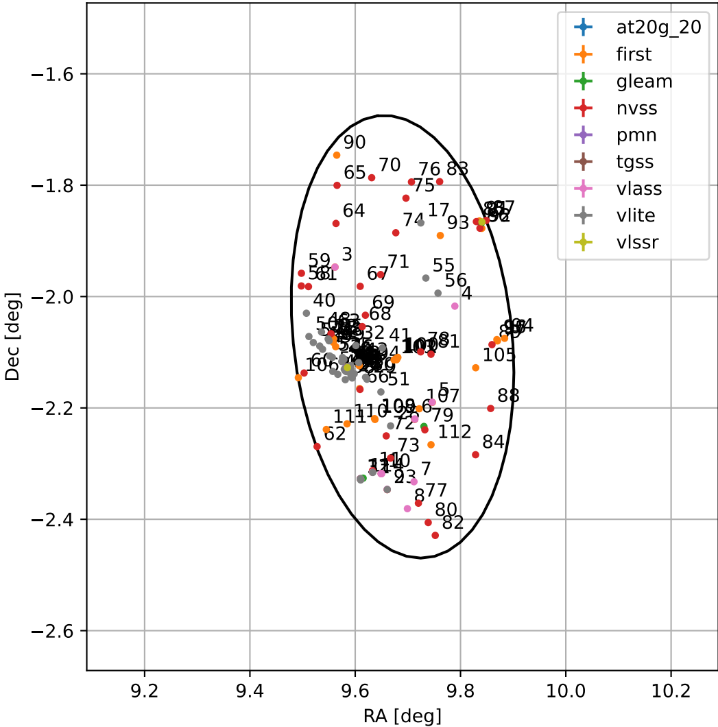
4FGL J0038.7-0204
