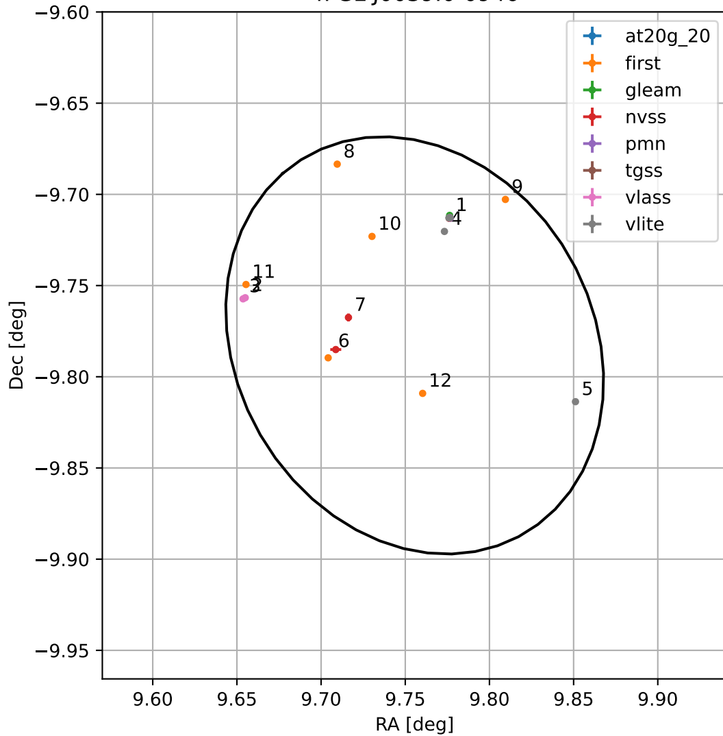
4FGL J0039.0-0946
