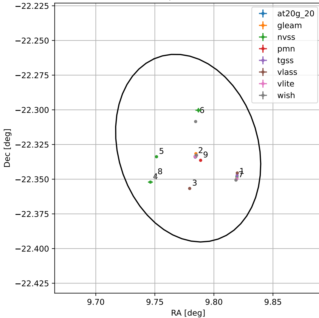
4FGL J0039.1-2219
