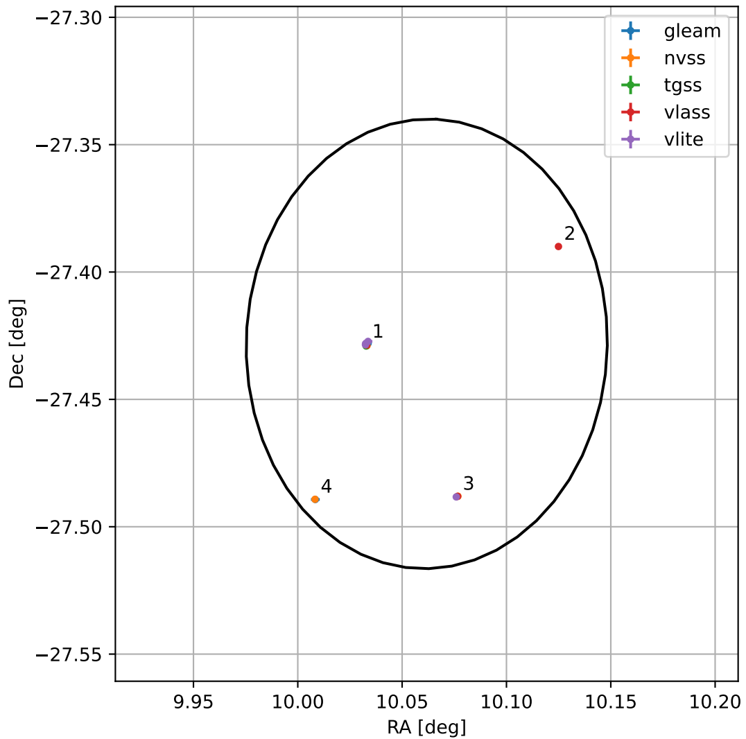
4FGL J0040.2-2725
