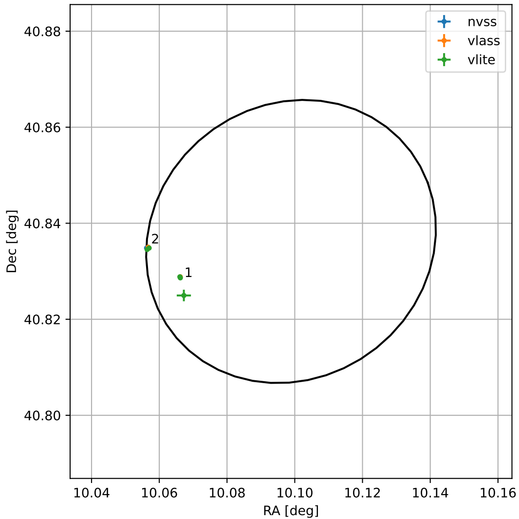
4FGL J0040.3+4050
