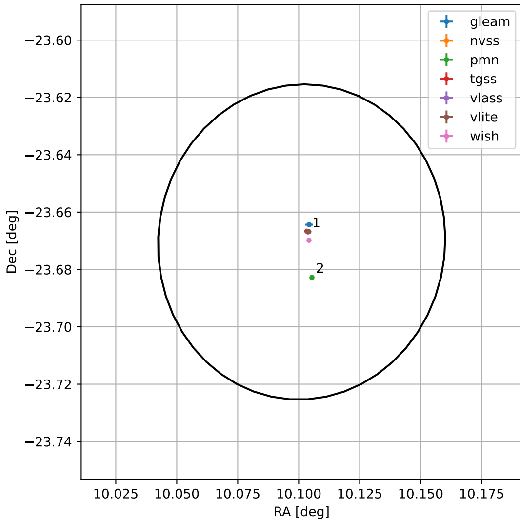
4FGL J0040.4-2340
