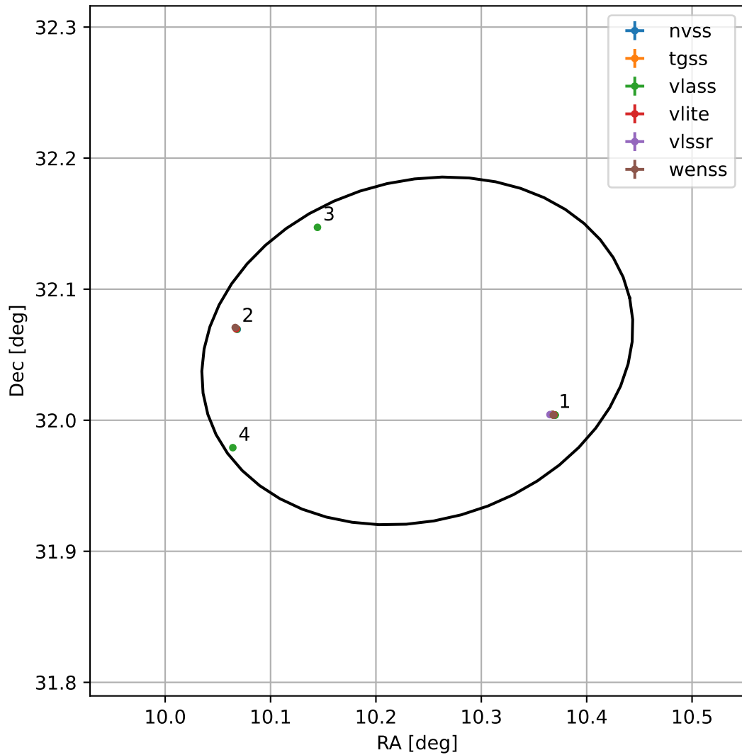
4FGL J0040.9+3203
