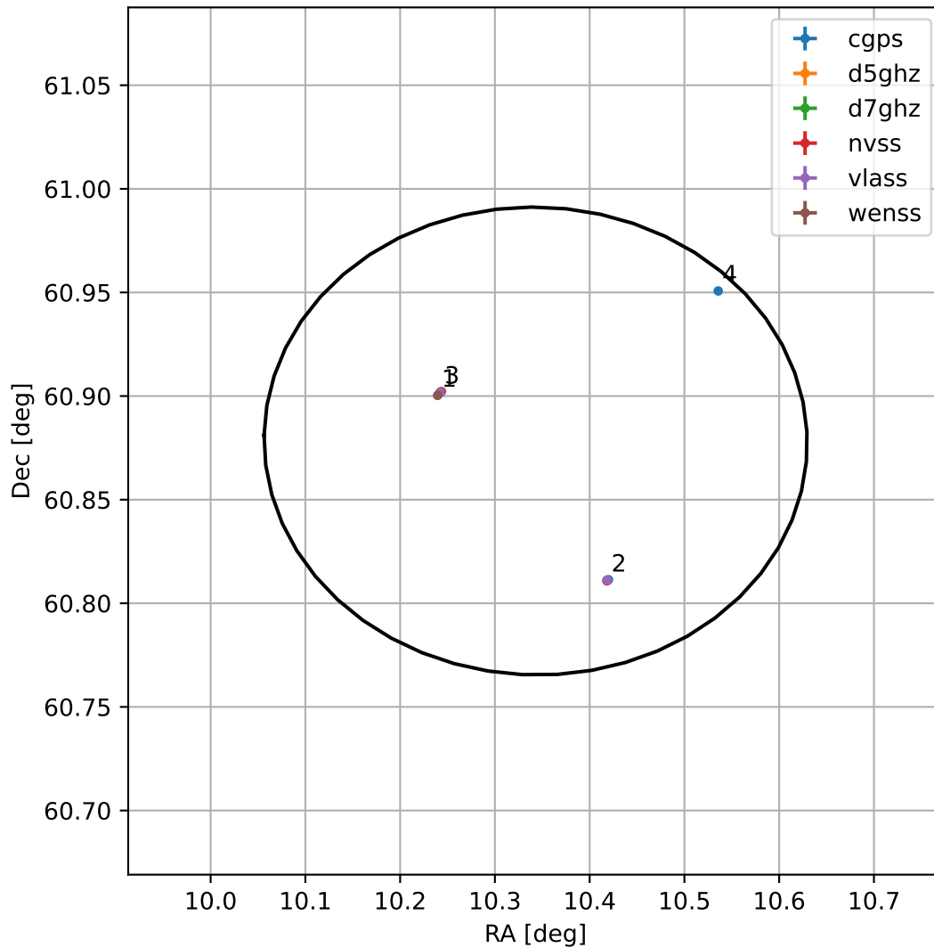
4FGL J0041.3+6052
