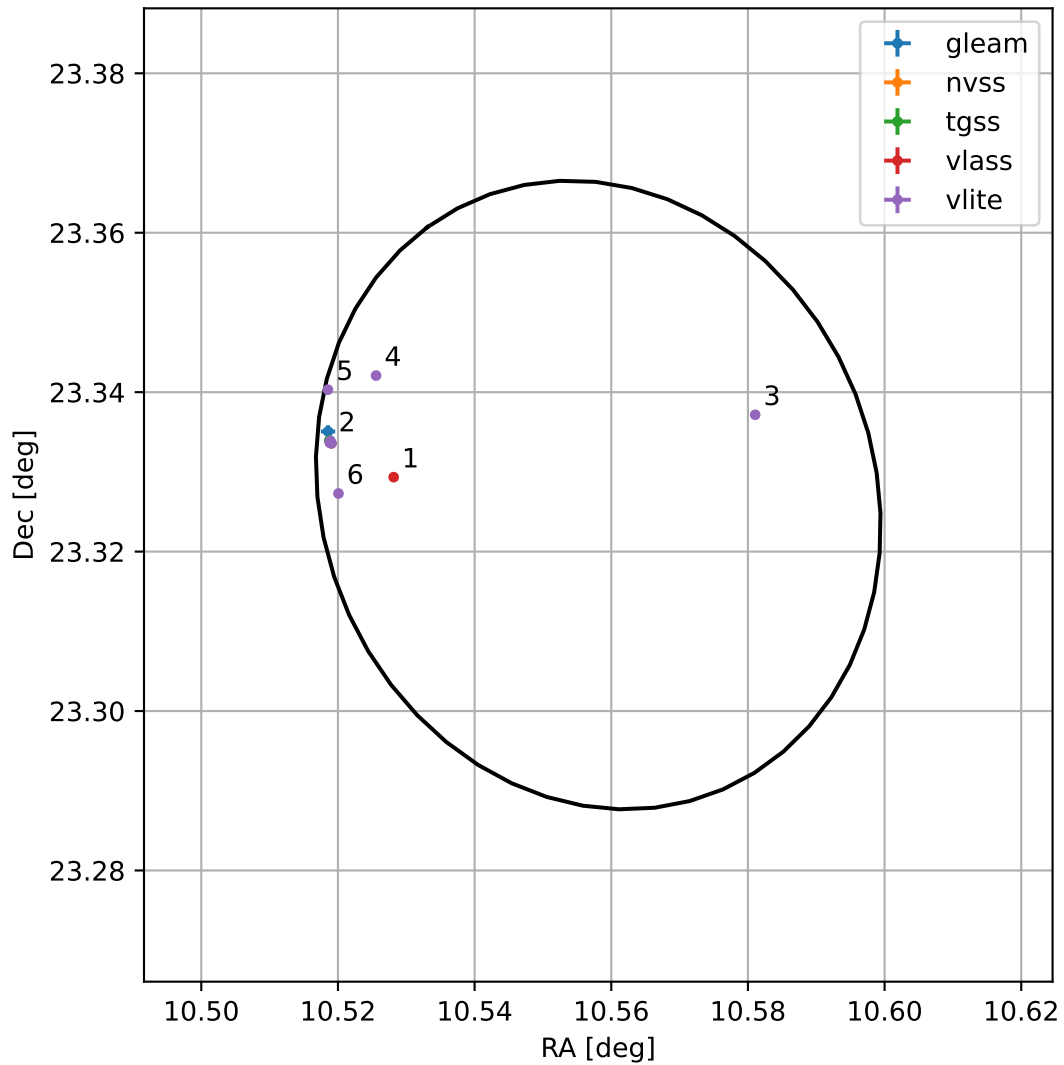
4FGL J0042.2+2319
