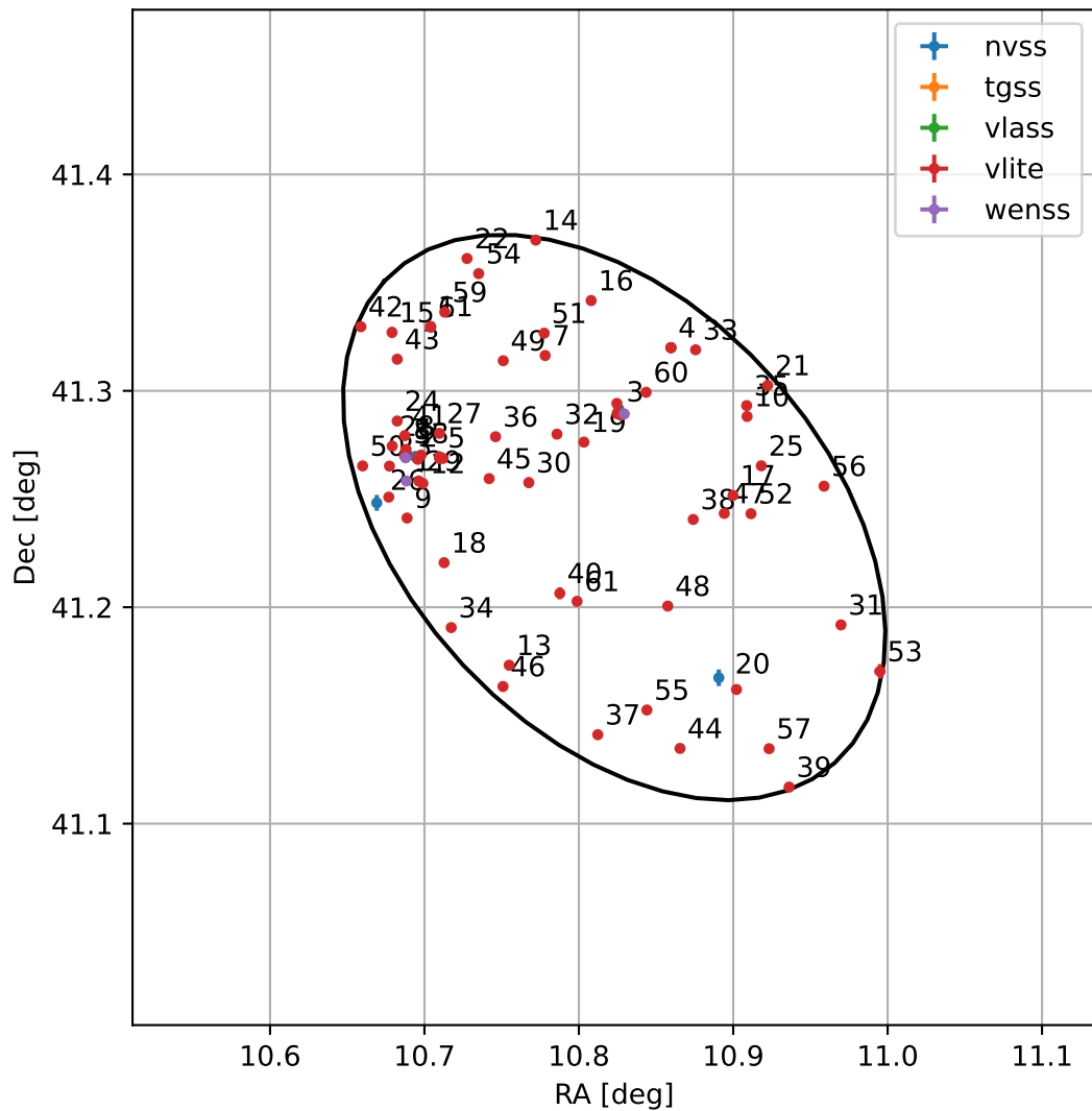
4FGL J0043.2+4114
