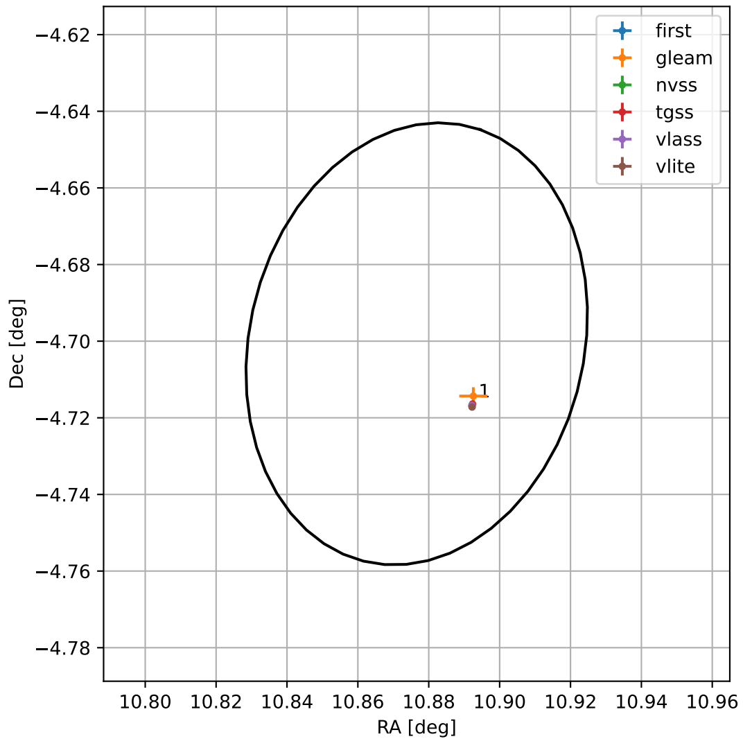
4FGL J0043.5-0442
